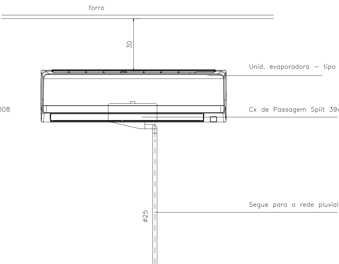
VISTA FRONTAL
