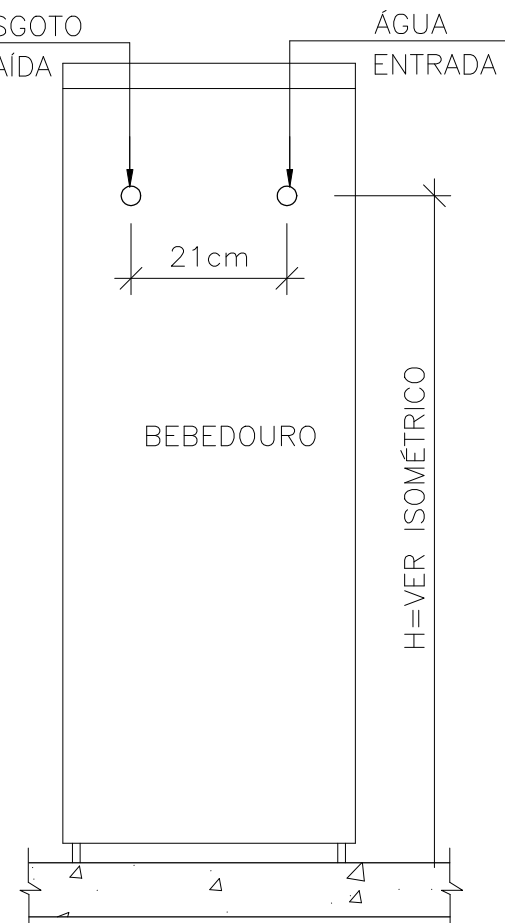
VISTA FRONTAL
