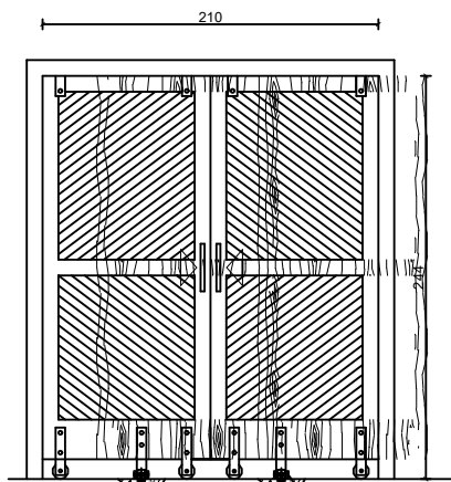
VISTA FRONT. PORTA DE CORRER (SALAS, BL. 1) Esc: 1/40
